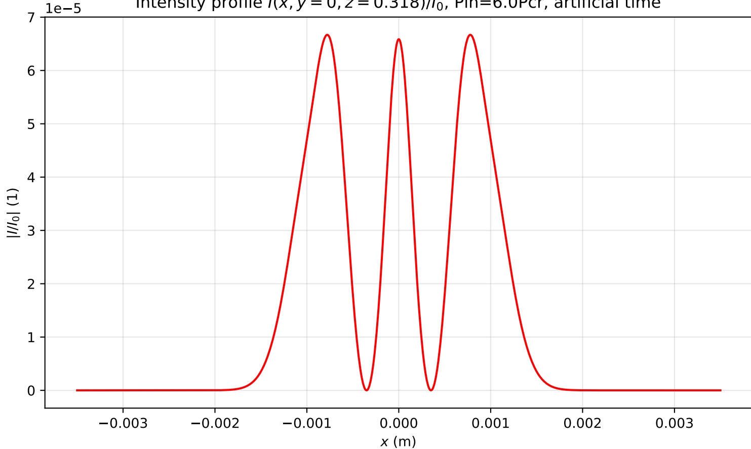
Intensity profile I(x, y = 0, z = 0.318)/I_0 , P_{in}=6.0P_{cr} , artificial time
